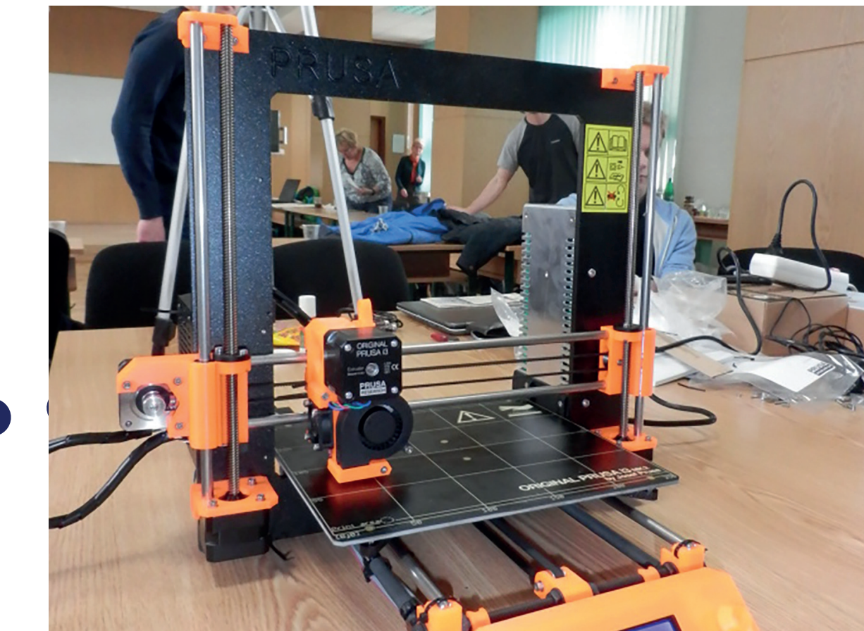
PRINTER ASSEMBLED
